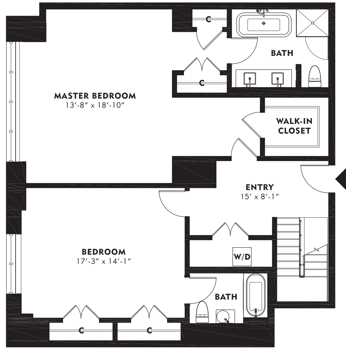
MEZZANINE LEVEL
