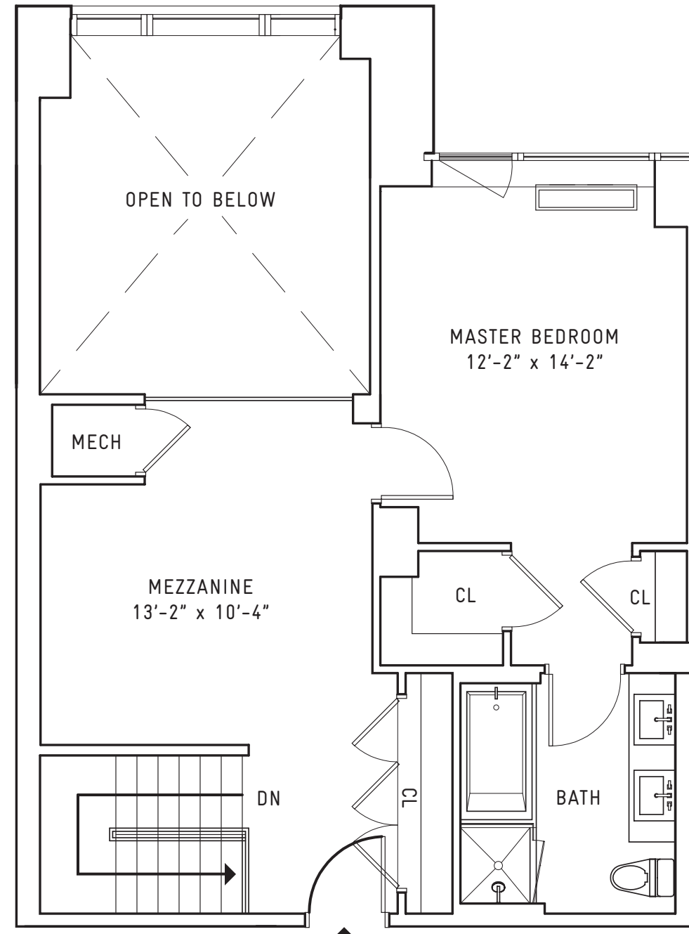
UPPER LEVEL
