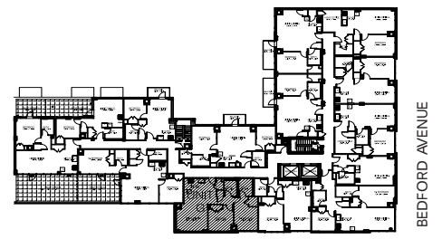
GATES AVENUE KEY PLAN
