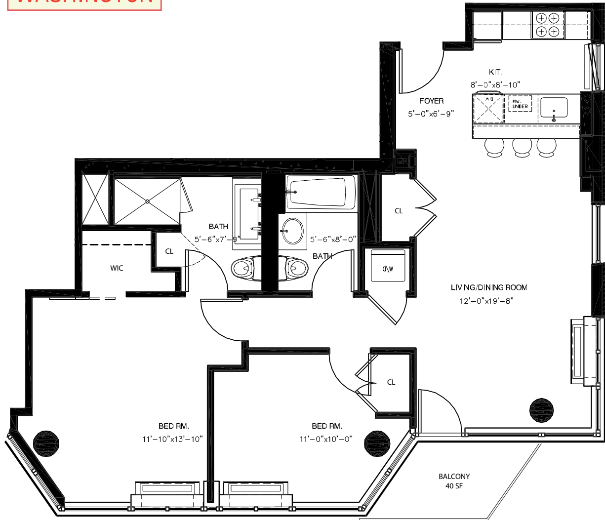
KEY PLAN
