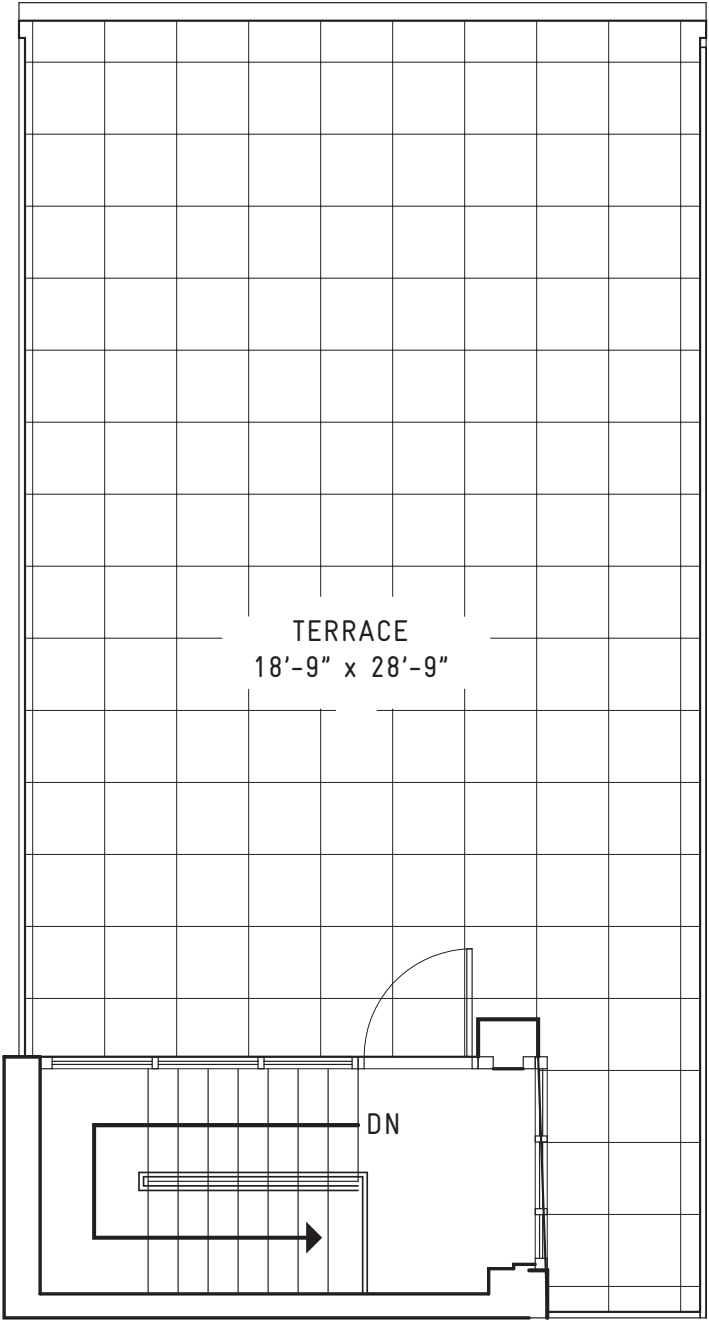
TERRACE LEVEL
