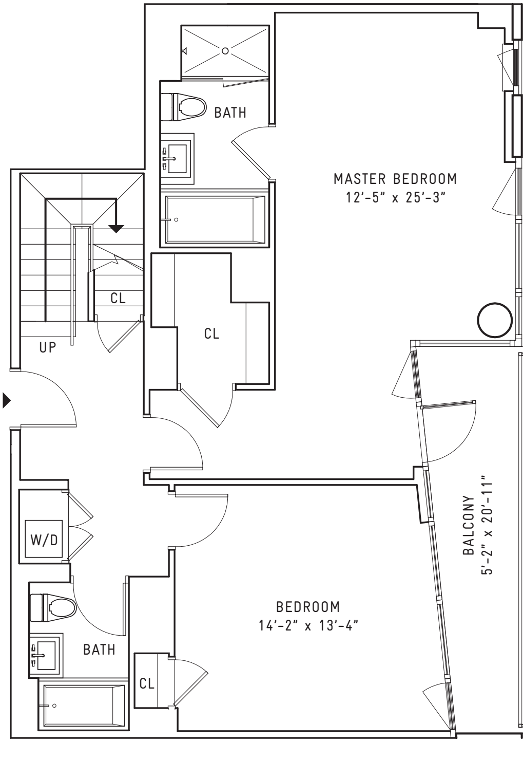
LOWER LEVEL
