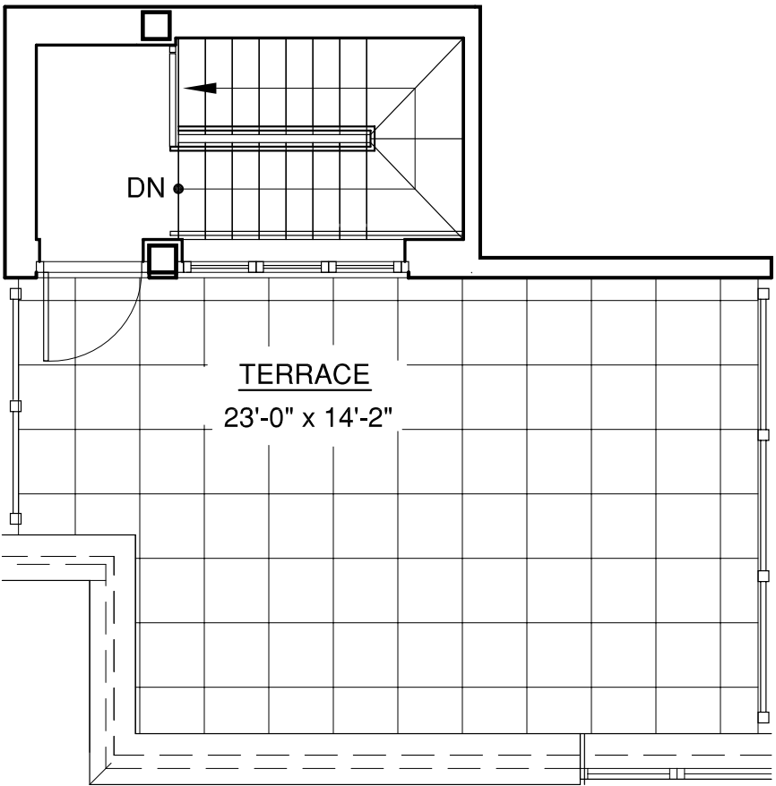
TERRACE LEVEL
