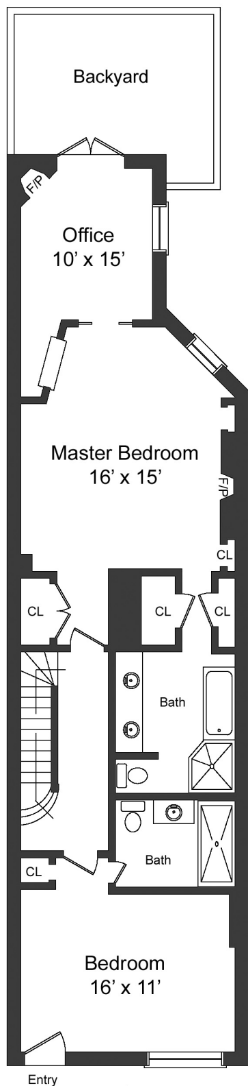
Ground Floor
