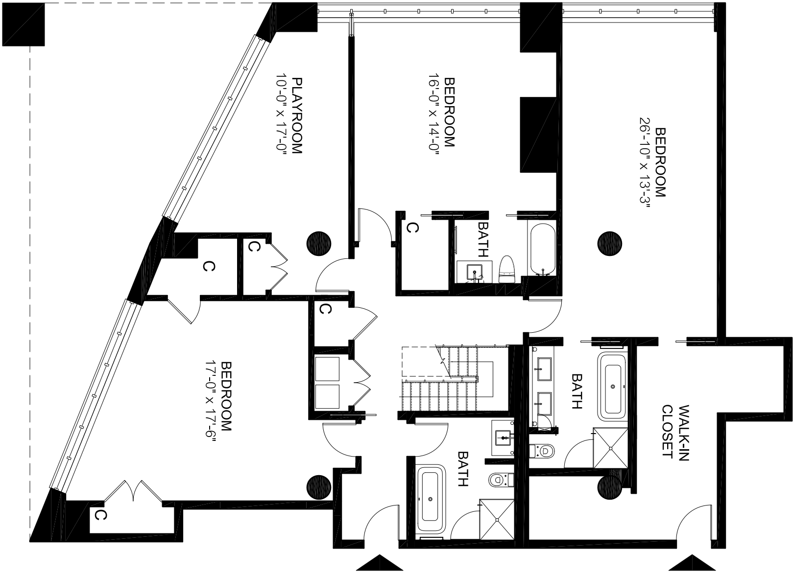
MEZZANINE
