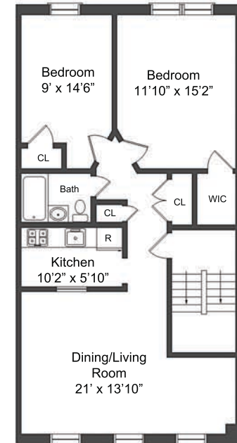
Fourth Floor
