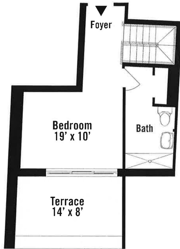
6th Floor
