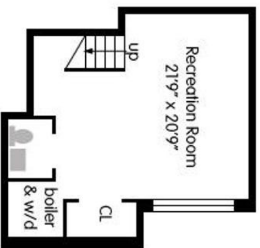
Lower Floor
