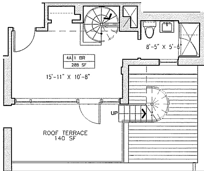
UPPER LEVEL 5TH FLOOR
