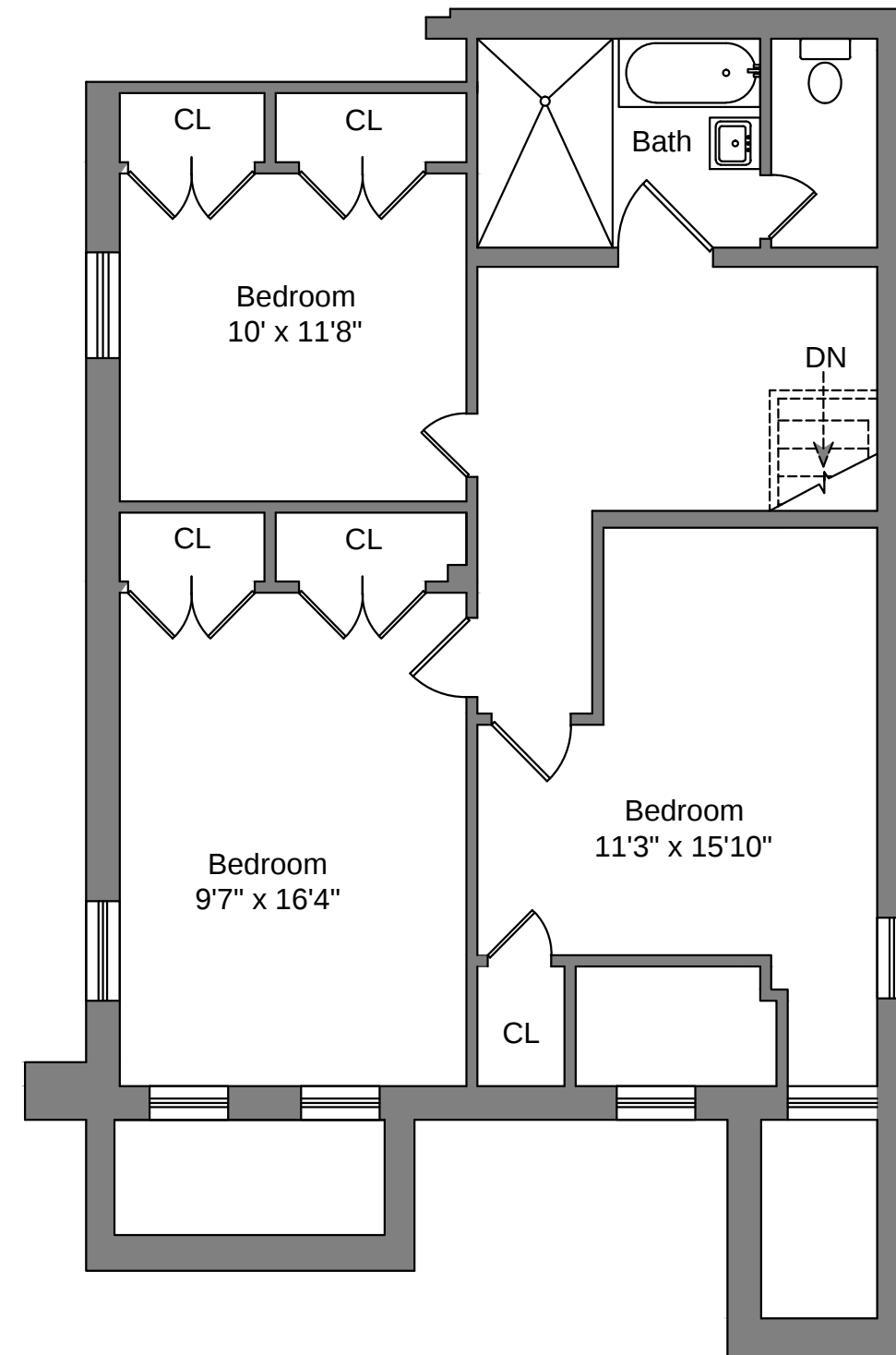
First Floor
