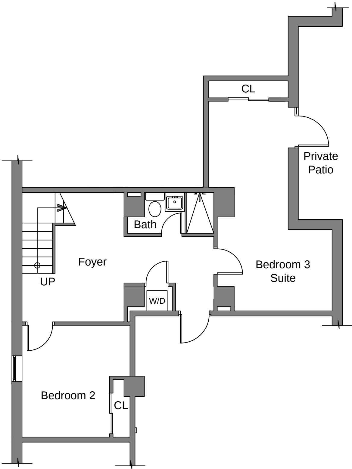
Basement
