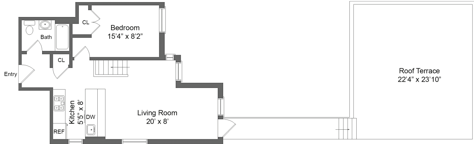
First Floor
