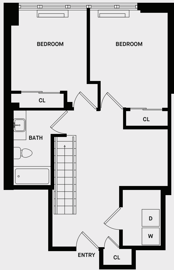
10TH FLOOR
