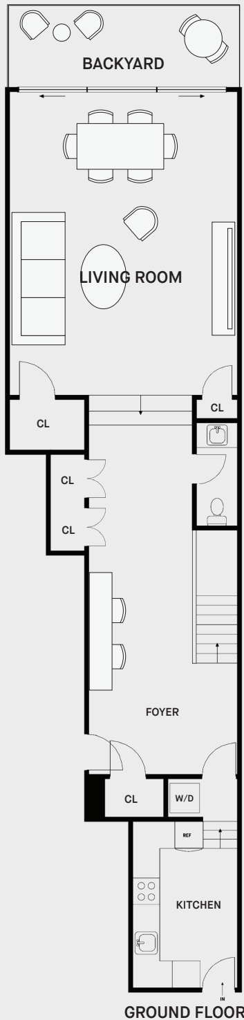
GROUND FLOOR
